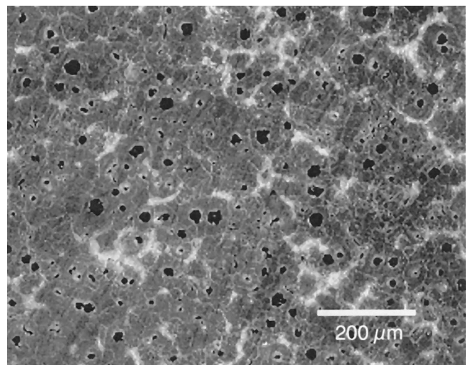
Figure 2 Microstructure of SiMo cast-iron at 700°C with pearlitic zone at grain boundaries. At room temperature lamellar pearlite became globular.
